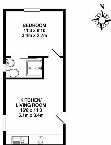
FLAT 4 LOWER BRISTOL ROAD, BATH, BA2 3BE TOTAL APPROX. FLOOR AREA 292 SQ.FT. (27.1 SQ.M.)
